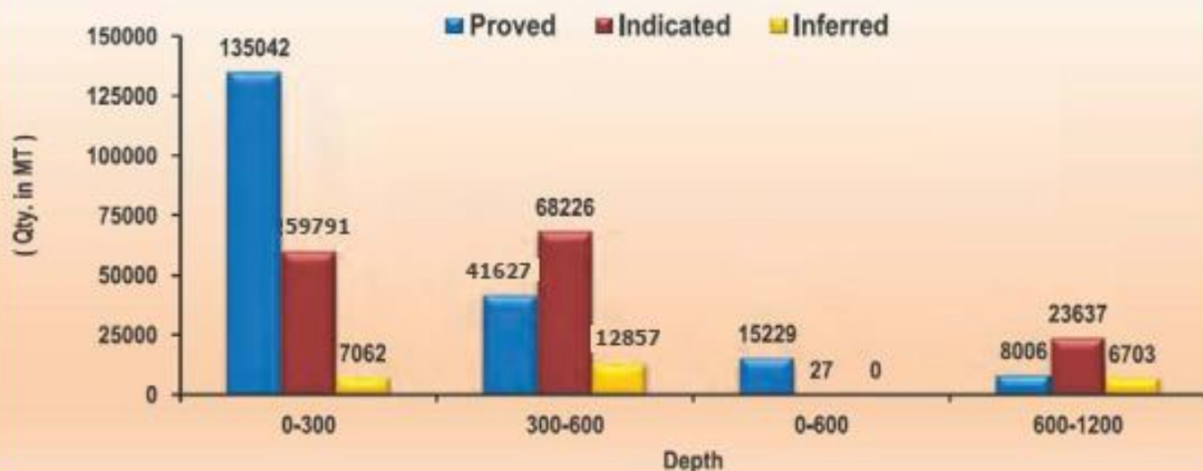
Depth Wise Inventory of Geological Resource of Coal in India (as on 1st April 2023)
