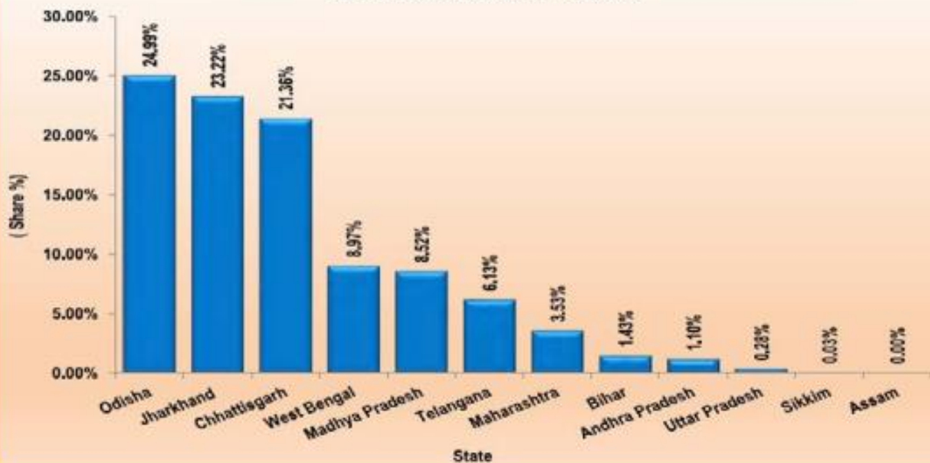
Share of State Wise Inventory of Geological Resource of Coal in Gondwana Coal Fields of India as on 01/04/2023
